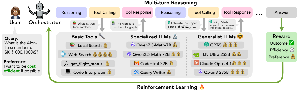
Figure 2 | Overview of Orchestrator. Given a task, Orchestrator alternates between reasoning and tool calling in multiple turns to solve it. Orchestrator interacts with a diverse tool set, including basic tools (web search, functions such as get_flight_status , etc.), specialized LLMs (coding models, math models, etc.) and generalist LLMs (GPT-5, Claude Opus 4.1, etc.). In training under ToolOrchestra, Orchestrator is jointly optimized by outcome, efficiency and preference rewards via reinforcement learning.
