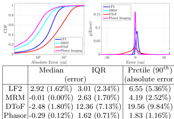
Fig. 4: The upper left panel shows the CDF of the depth error for LF2, MRM, DToF, and Phasor, for simulated data from FLAT, affected by shot noise and MPI. The upper right panel shows the histogram of the error. All pixels whose real depth is in the [1.5m, 5m] range have been considered. Our MRM outperforms LF2 and DToF, and it comes much closer to the accuracy achieved using the MPI-dedicated, higher-frequency modulations of Phasor. The table shows corresponding median and Inter Quartile Range (IQR) of the depth error, and 90 th percentile of the absolute error, in cm. The numbers in the brackets indicate the relative errors.
